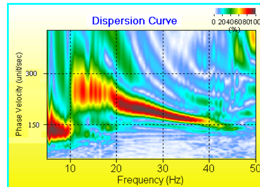
Figure 3. Rayleigh-wave dispersion curve analysis image of phase-velocity versus frequency domain.
