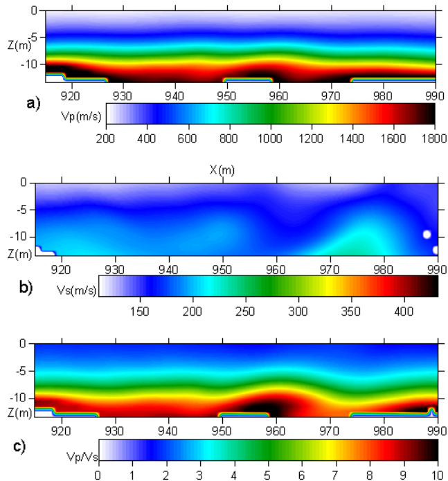
Figure 2. Refraction tomography solutions for the second levee site. a) P-wave, b) S-wave, and c) V_p/V_s ratio
