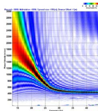
Figure 10. Dispersion-curve image of the synthetic seismic record from the 10-layer model between 13-45 Hz.
