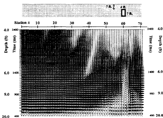
Figure 4. Stacked section of shot gather after dynamic linear move out (DLMO) correction.
