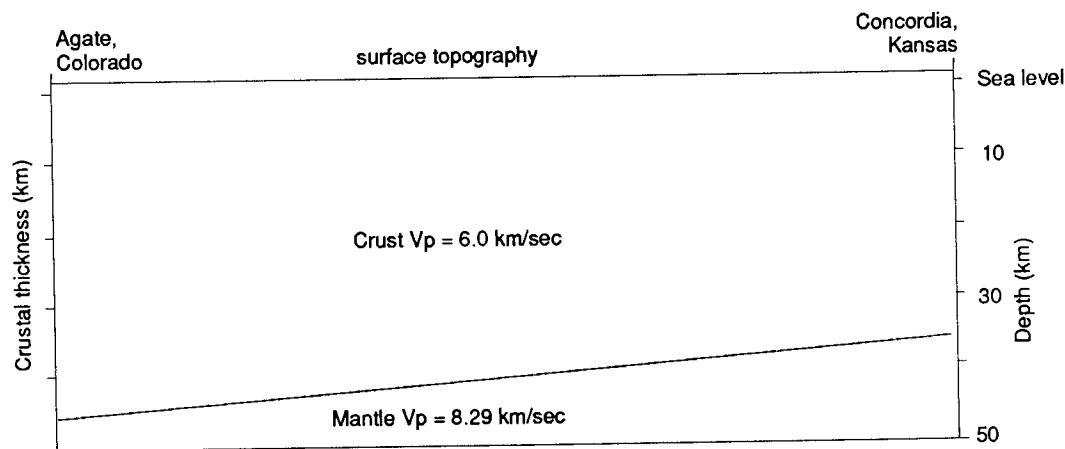
FIGURE 7—CROSS SECTION SHOWING CRUSTAL THICKNESS, AVERAGE VELOCITY OF THE CRUST, AND VELOCITY OF THE UPPER MANTLE. This cross section directly correlates to the regional gravity-gradient plot of fig. 8.
